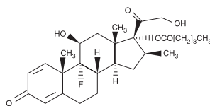
Betamethasone valerate
